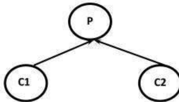
Hierarchical Inheritance
